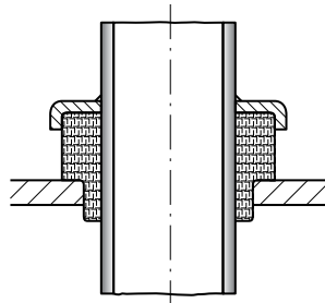
Pipe isolation
